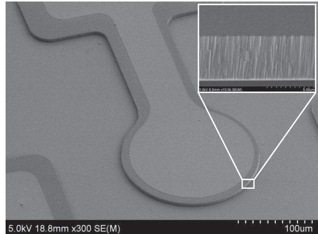
Fig. 3 SEM image of thin film actuator and cross section of thin piezo film.
