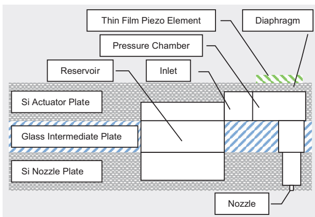
Fig. 2 Cross section of an individual channel of the thin film MEMS head.
