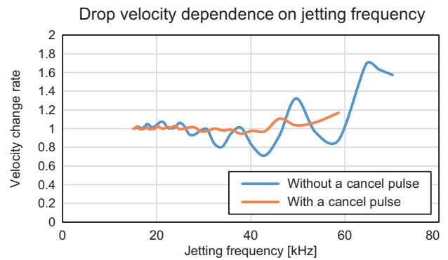
Fig. 11 Drop velocity dependence on jetting frequency.
