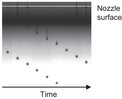
Fig. 7 Sequential stroboscopic image of droplet.
