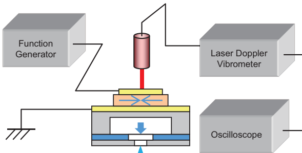
Fig. 8 Schematic image of actuator oscillation observation system.
