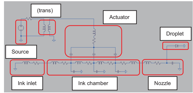
Fig. 5 Equivalent circuit model (basic model).
