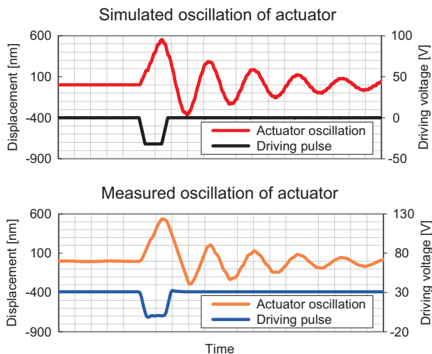
Fig. 9 Calculated diaphragm oscillation (top) and measured one (bottom).
