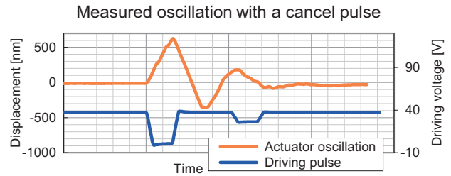
Fig. 10 Measured oscillation with cancel pulse.
