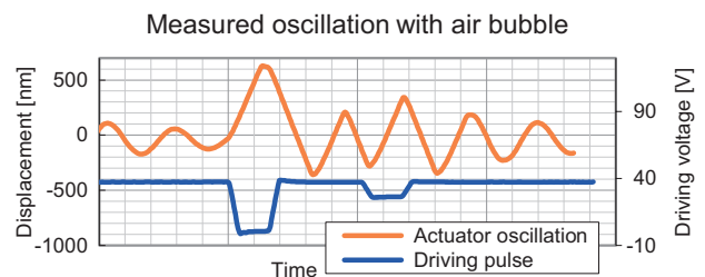
Fig. 12 Measured oscillation disturbed by an air bubble.
